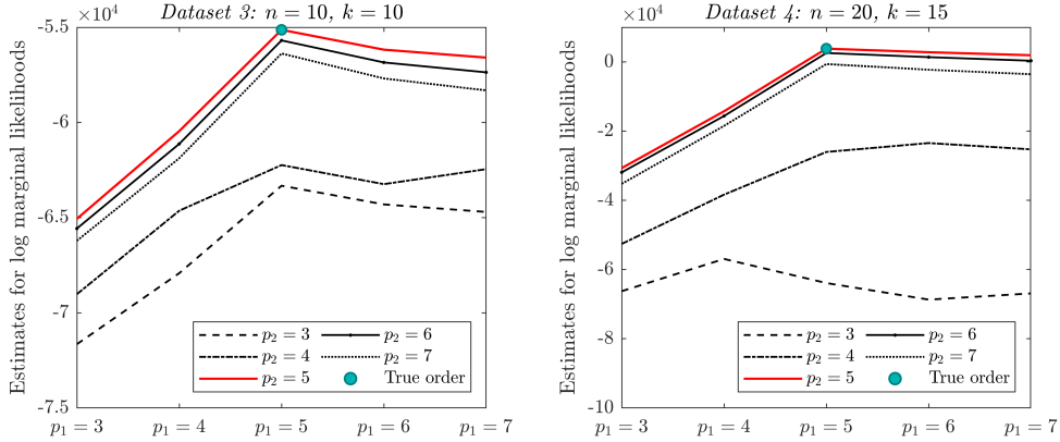
Figure 4: Estimates for log marginal likelihoods when true order of the factor matrix is p_1 = 5, p_2 = 5
